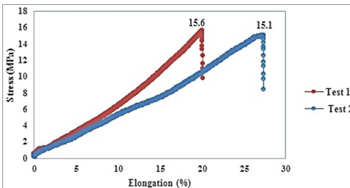
Figure 2. Stress-Elongation curves (n=2) for verification of the optimal conditions.
