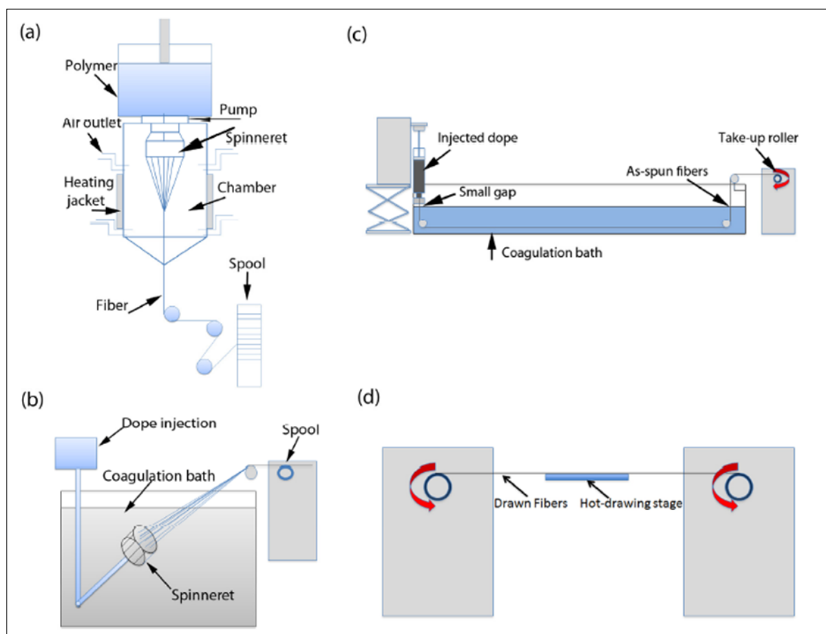
Figure 1. Schematics for the different fibre preparing techniques (a) dry-turning; (b) wet-turning; (c) dry-stream wet or gel turning; and (d) post-handling by hot-arrange drawing [ 10].
