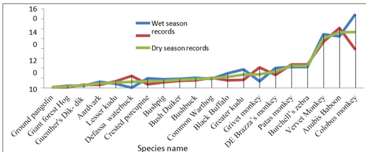
Figure 7. Mean number of species richness and frequency of records computed by rarefaction curve two seasons.
